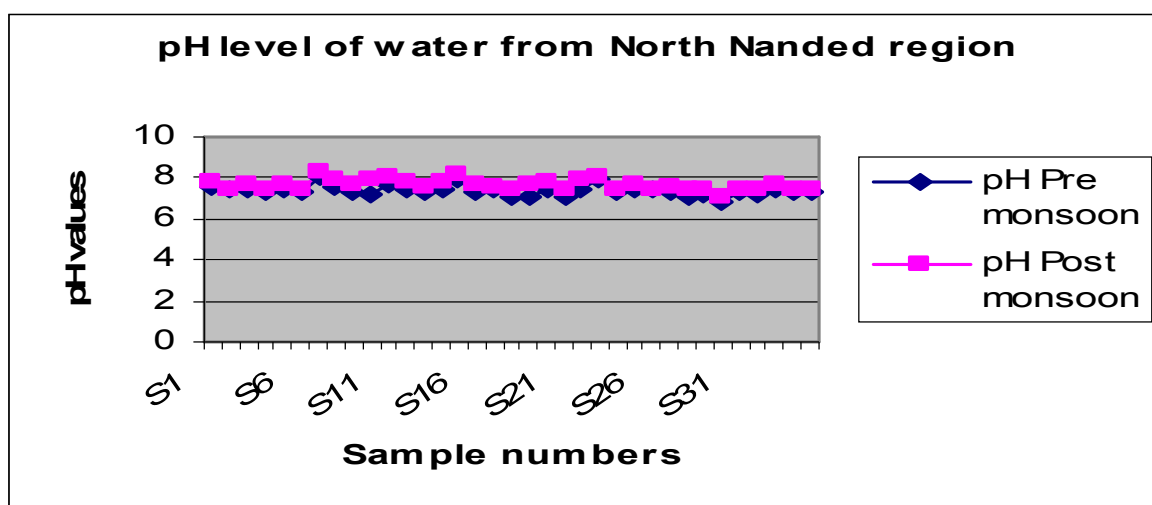
Figure 4. The pH variations from the selected stations.
