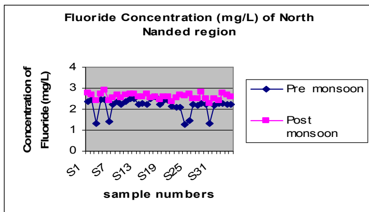
Figure 3. Fluoride variations on water from the selected sites.
